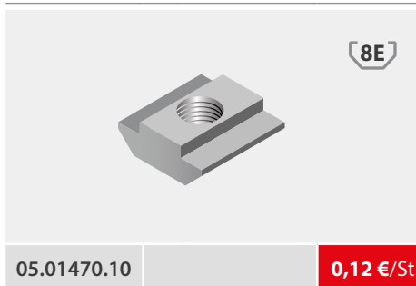
Nutenstein, T-Form • 8E | M6 | 16 mm, vz.
