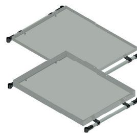
Ablagetasse waagrecht B x T = 605 x 405
